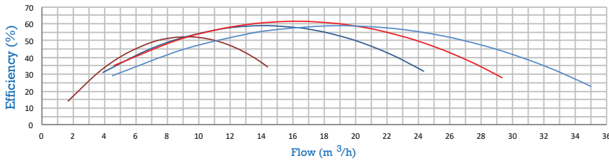
Hydraulic Performance
