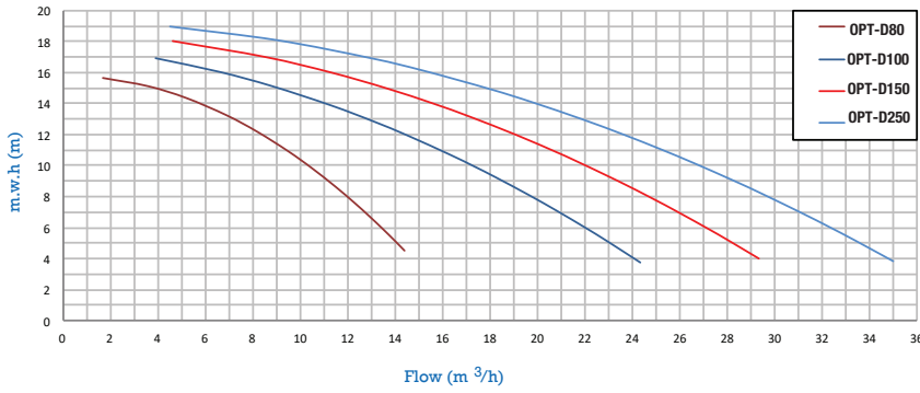
Characteristics curve
